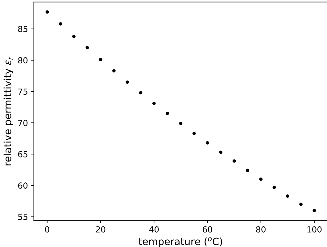
relative permittivity of water vs. temperature
